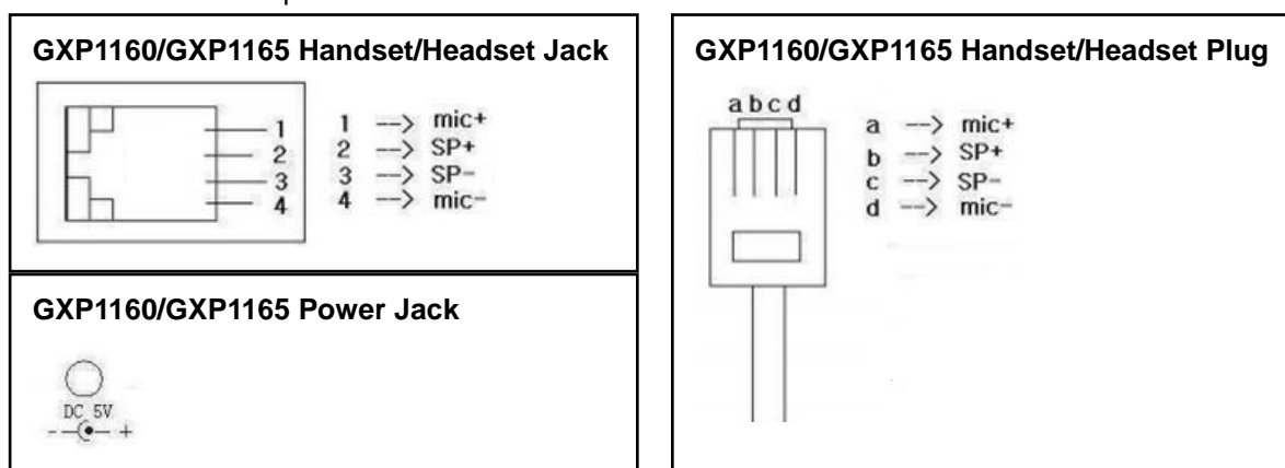
Figure 2: GXP1160/GXP1165 Pin-out
