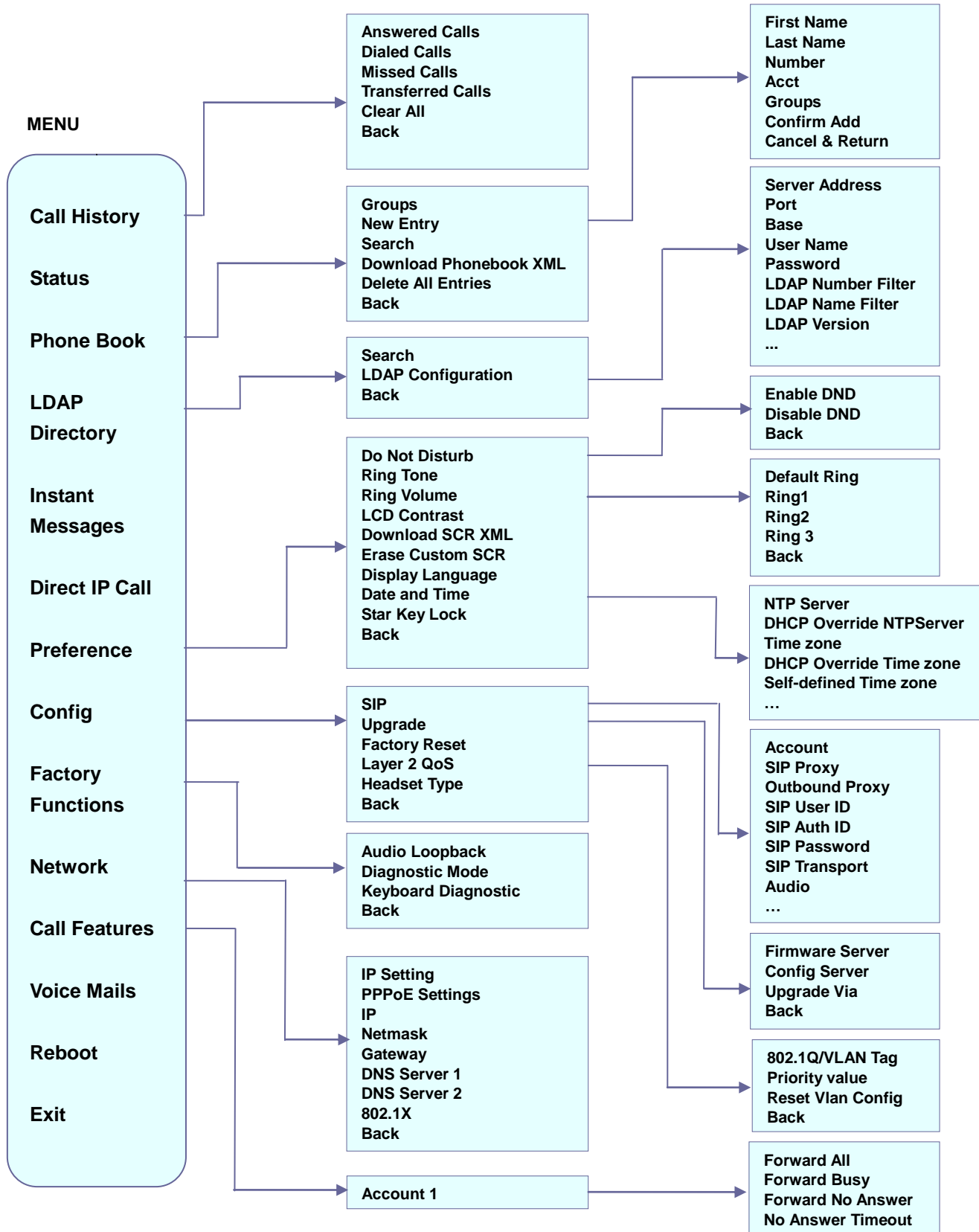
Figure 4: Keypad MENU Flow
