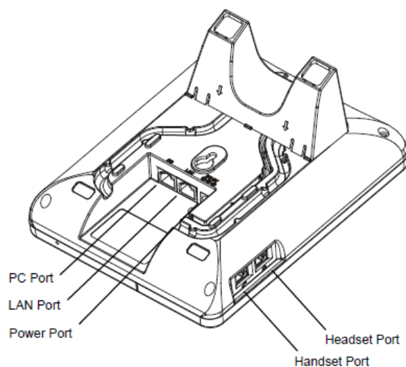
Figure 1: GXP1160/GXP1165 Ports
