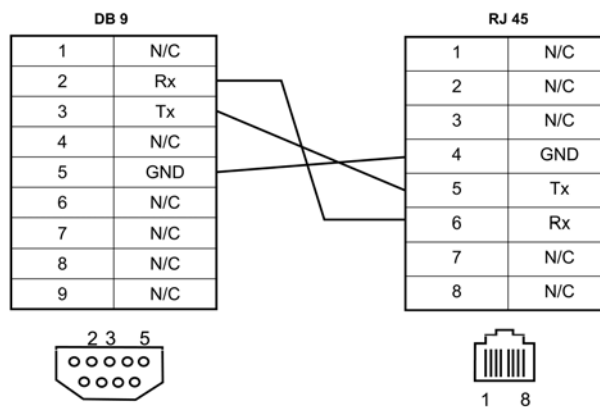
Figure 3. Console pinout
