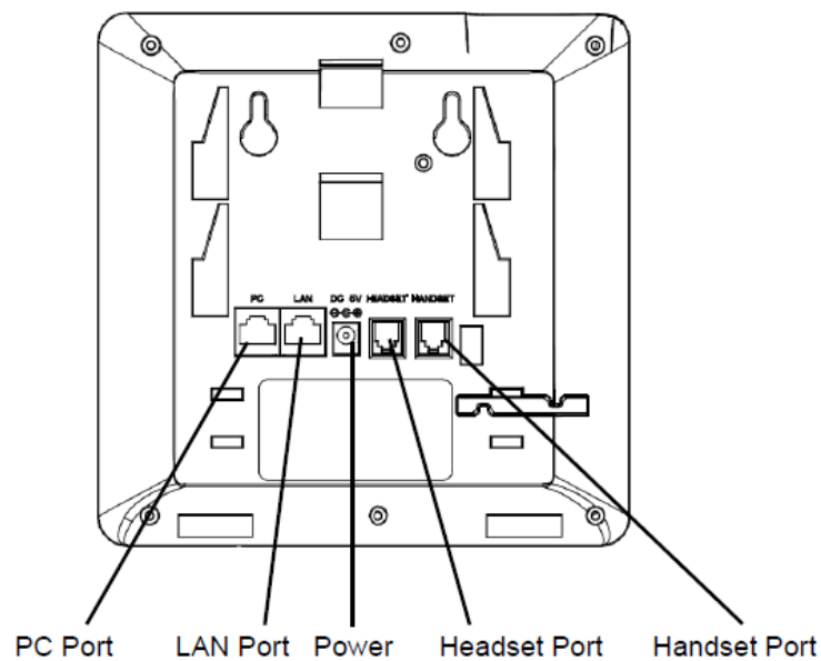
Figure 1: GXP1400/GXP1405 Ports
