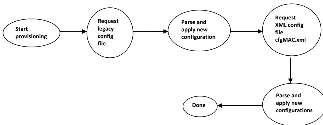
Figure 1: Provisioning Flow.
